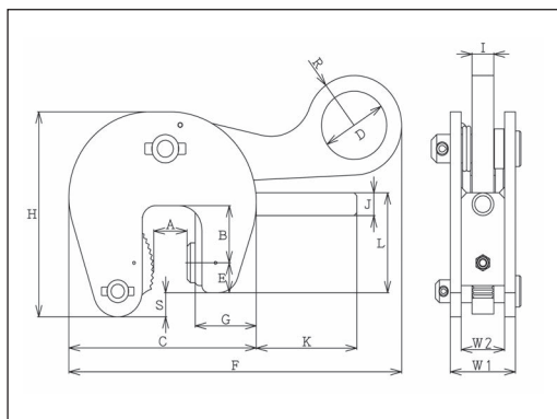
■Table of Dimensions (Model : AC)
