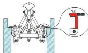
Variable (free gradient) roadside ditch
