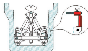
U-shaped channel
