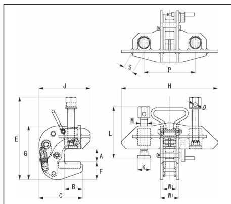
■ Table of Dimensions (Model : ALB)
