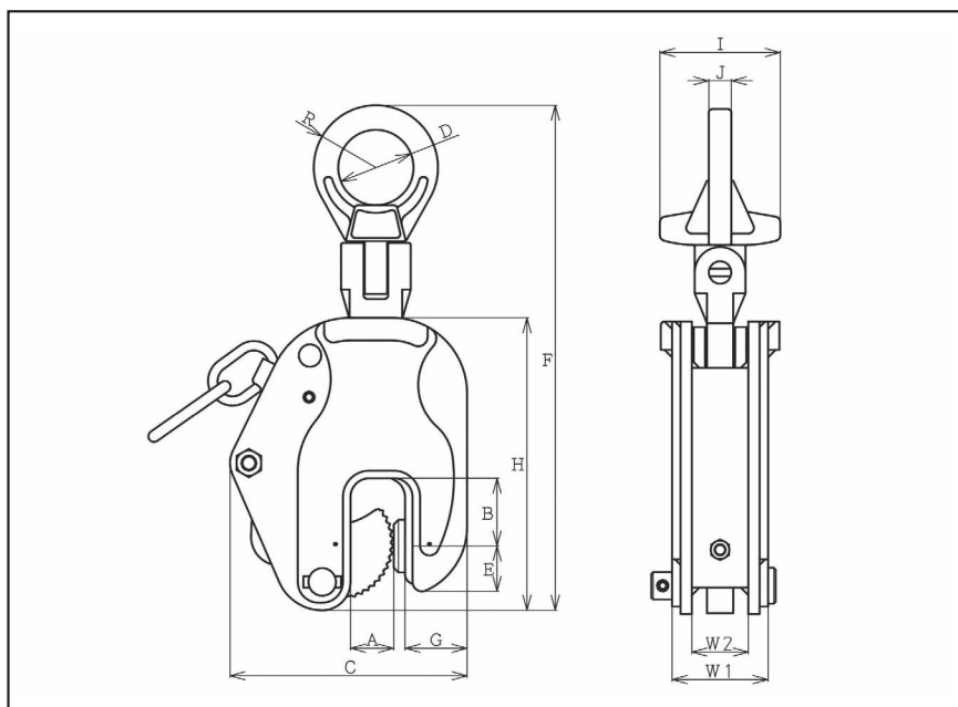
■Table of Dimensions (Model : ET)
