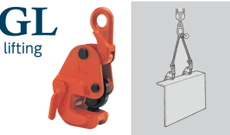
Models AMS/AMN Lateral lifting clamps P.18
