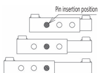
Lifting width adjustment mechanism
