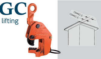
Model GD Lateral lifting clamp P.17
