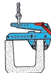
▲ U-shaped reinforced concrete channels ▲ Varying thickness U-shaped channels
