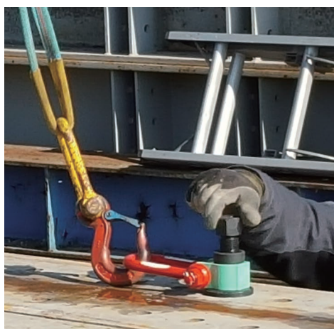
Can be tightened from the outside of objects to be lifted
