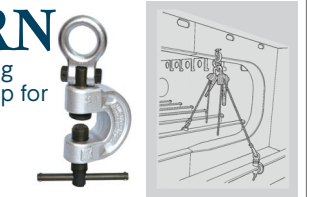
Model SARO Non-marring screw clamp for pulling P.26
