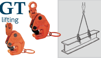
Model GC Lateral lifting clamp P.16
