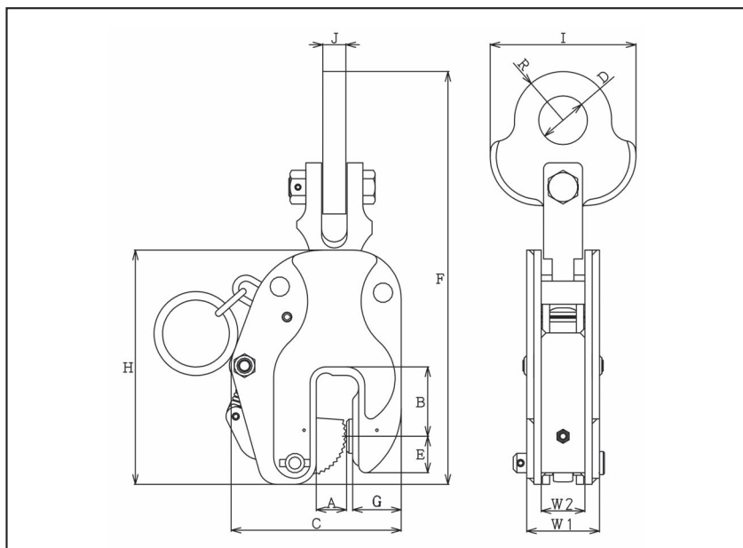
■Table of Dimensions (Model : SLT)
