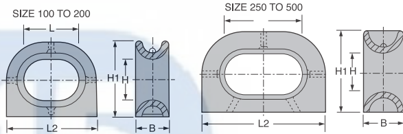
\\ JIS F-2005 CLOSED CHOCKS DECK MOUNTING (클로즈 초크)
